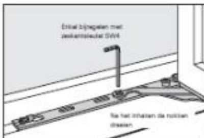
Hooklager R
